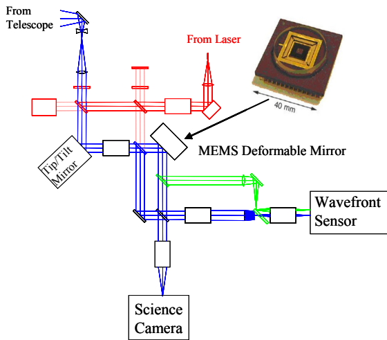
Figure 1. MEMS-AO / ViLLaGEs system. This system employs a 140 actuator MEMS deformable mirror and fits on the back of the Lick Observatory 40-inch Nickel telescope.
